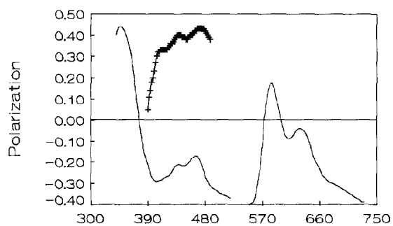
Figure 3. [\text{Ru}(\text{bpy})(\text{py})_4](\text{ClO}_4)_2 EtOH
