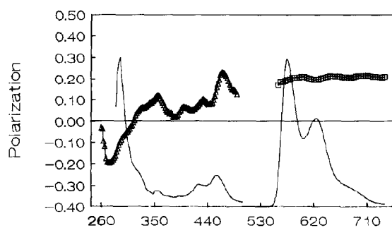
Figure 4. [\text{Ru}(\text{bpy})_3]^{2+} in EtOH at 77K
