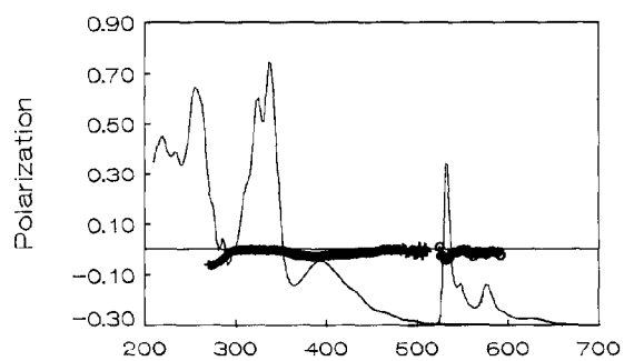
Figure 6. [\text{Ru}(\text{ibiq})_3](\text{PF}_6)_2 in EtOH
