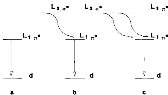
Fig. 2. Orbital Arrangements of Monomeric Complexes Three possible arrangements which produce monomeric or pseudo-monomeric complexes. (a). A true monomeric complex with only a single diimine chelate ligand. (b). A second diimine chelate with a \pi^* orbital at much higher energy produces a pseudo-monomeric complex luminescing from the lowest-lying chromophore. In (c), this is extended with two additional diimine chromophores whose \pi^* orbitals are significantly higher in energy.
