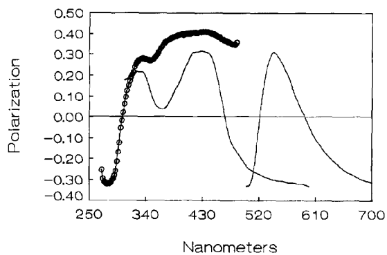
Figure 5. \text{K}_2[\text{Ru}(\text{bpy})(\text{CN})_4] EtOH 77K
